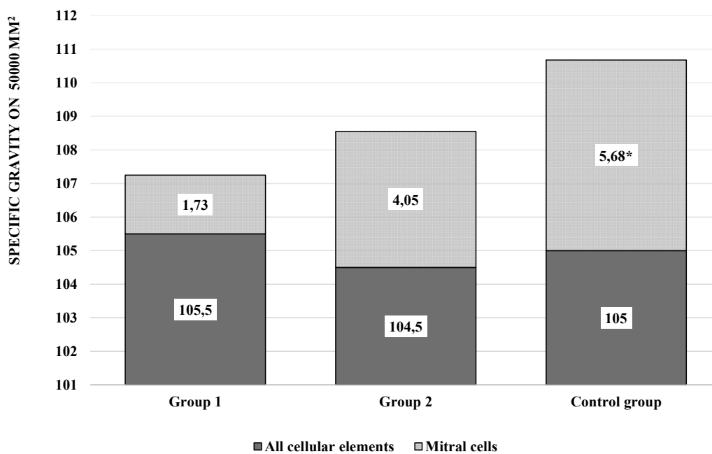
Fig. 3. Specific gravity of cellular elements in human OB (* – p \leq 0.05 relative to group 1)
